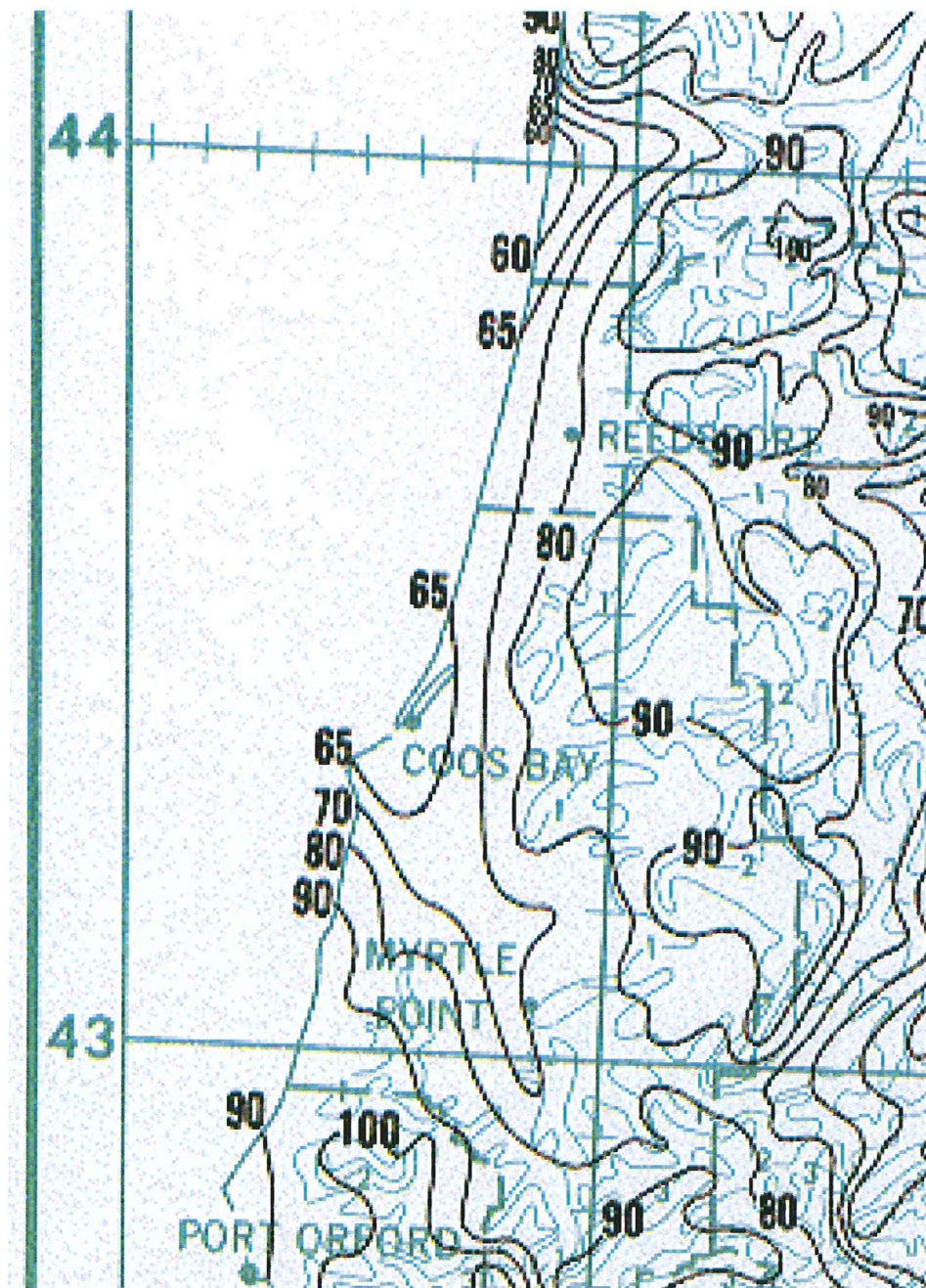
Isopluvials of 100-year 24-hour Precipitation In tenths of an inch
