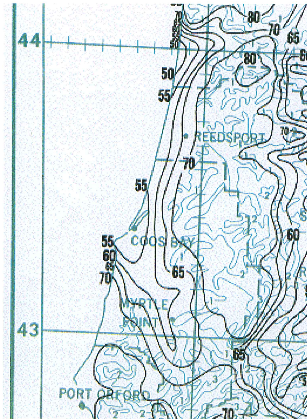
Isopluvials of 25-year 24-hour Precipitation In tenths of an inch
